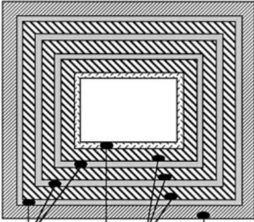
3 insulating layers of high dielectric composition Interior ferromagnetic sheet metal Steel wool layers Final high dielectric exterior layer
